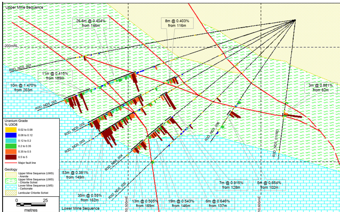
Figure 2 – Interpreted cross section showing the drilling results from NDD5. (Includes gamma and chemical assay results)
