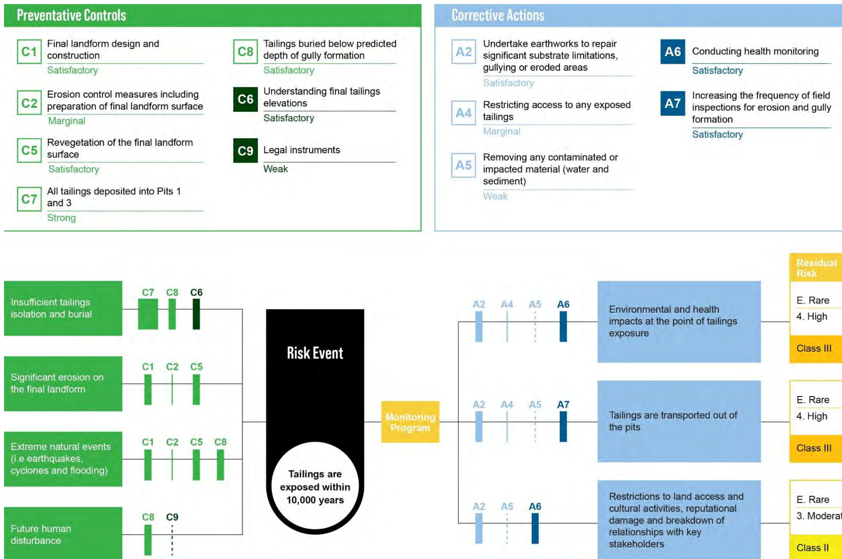
Figure 6-7: Bow-tie diagram for tailings isolation (L2)
