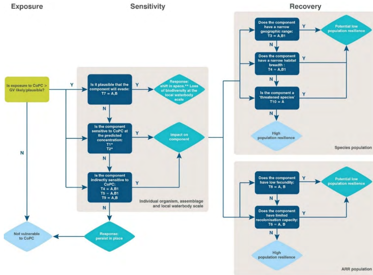
Figure 7-13: Decision tree for vulnerability assessment framework
