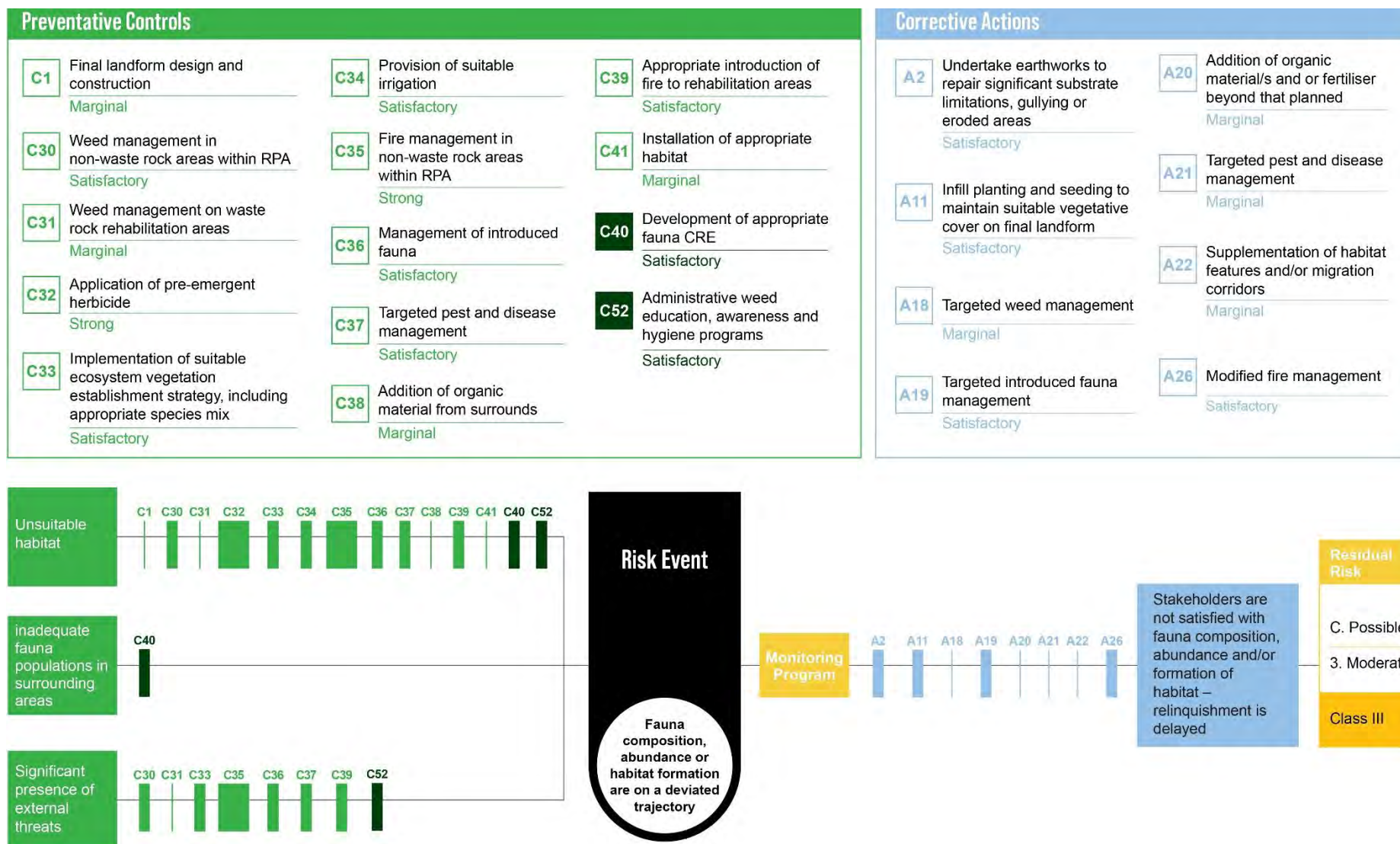
Figure 9-4: Bow-tie diagram for fauna composition, abundance or habitat formation (ES2)
