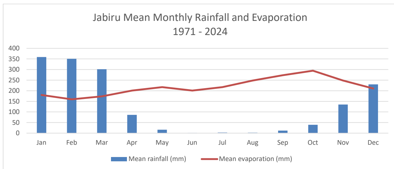
Figure 2-1: Jabiru mean monthly rainfall and evaporation (1971 to 2024: BoM 2024)
