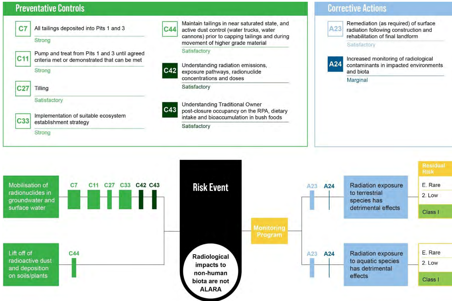
Figure 10-3: Bow-tie diagram for radiation doses to non-human biota (plants and animals) (R2)
