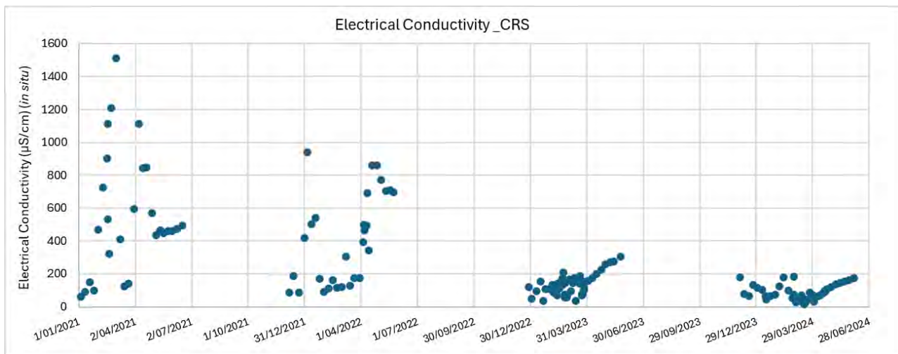
Figure 7-6: Pit 1 - CRS water quality data – Electrical Conductivity
