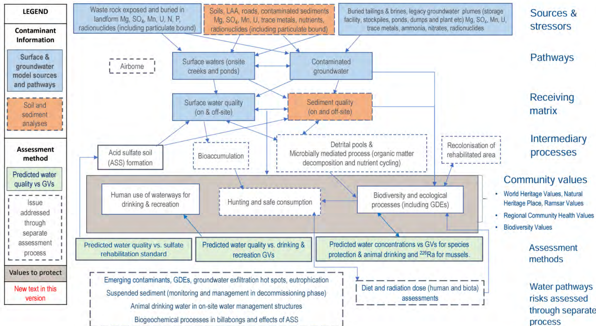
Figure 7-12: Conceptual model underpinning the APRA (BMT, 2023a)
