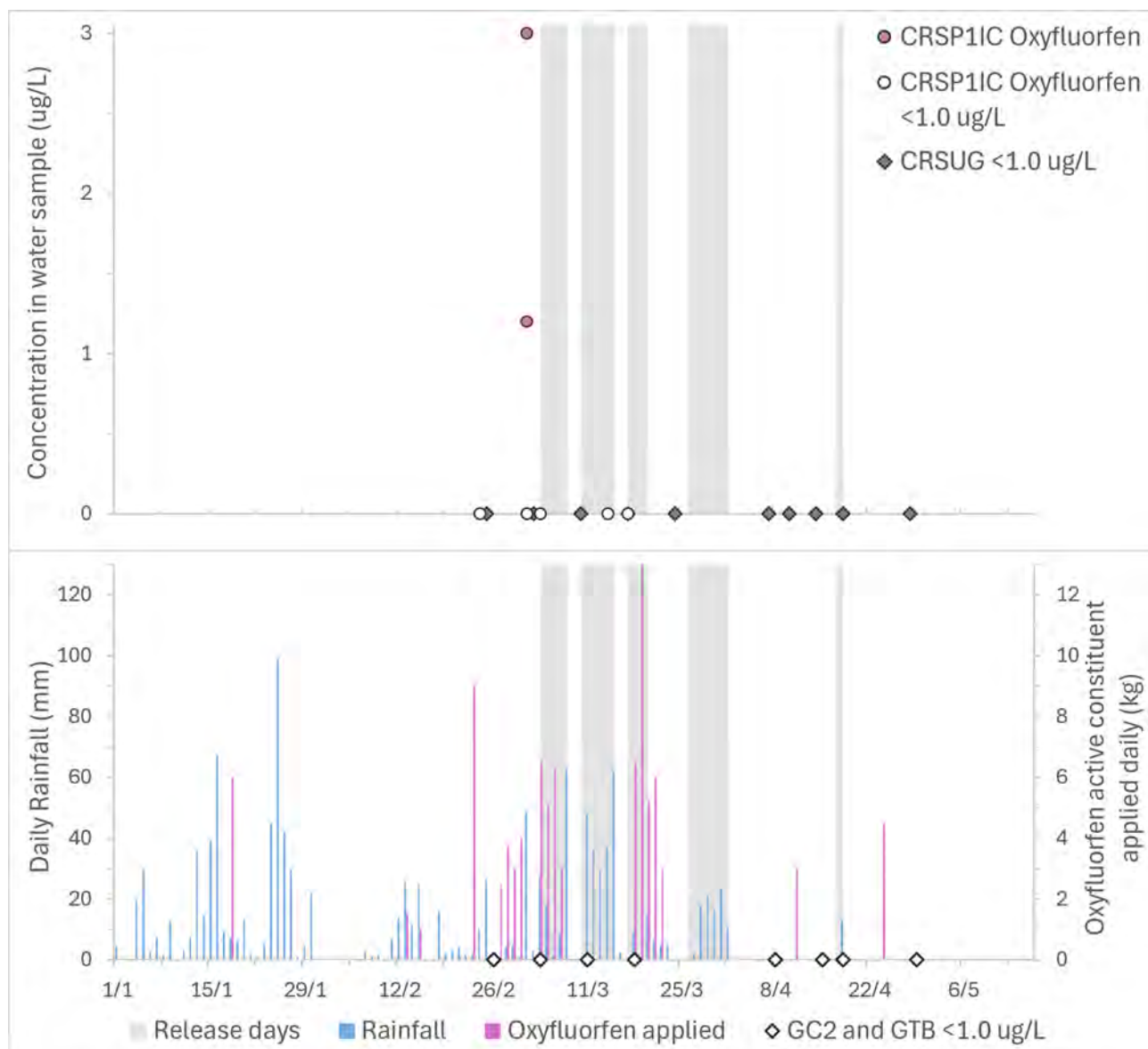
Figure 7-10: Daily rainfall (Jabiru airport) and estimated oxyfluorfen applied daily in the Pit 1/CRS catchment from 1 Jan to 16 May 2024 (bottom). Oxyfluorfen concentrations at CRSUG and CRSP1IC (top).
