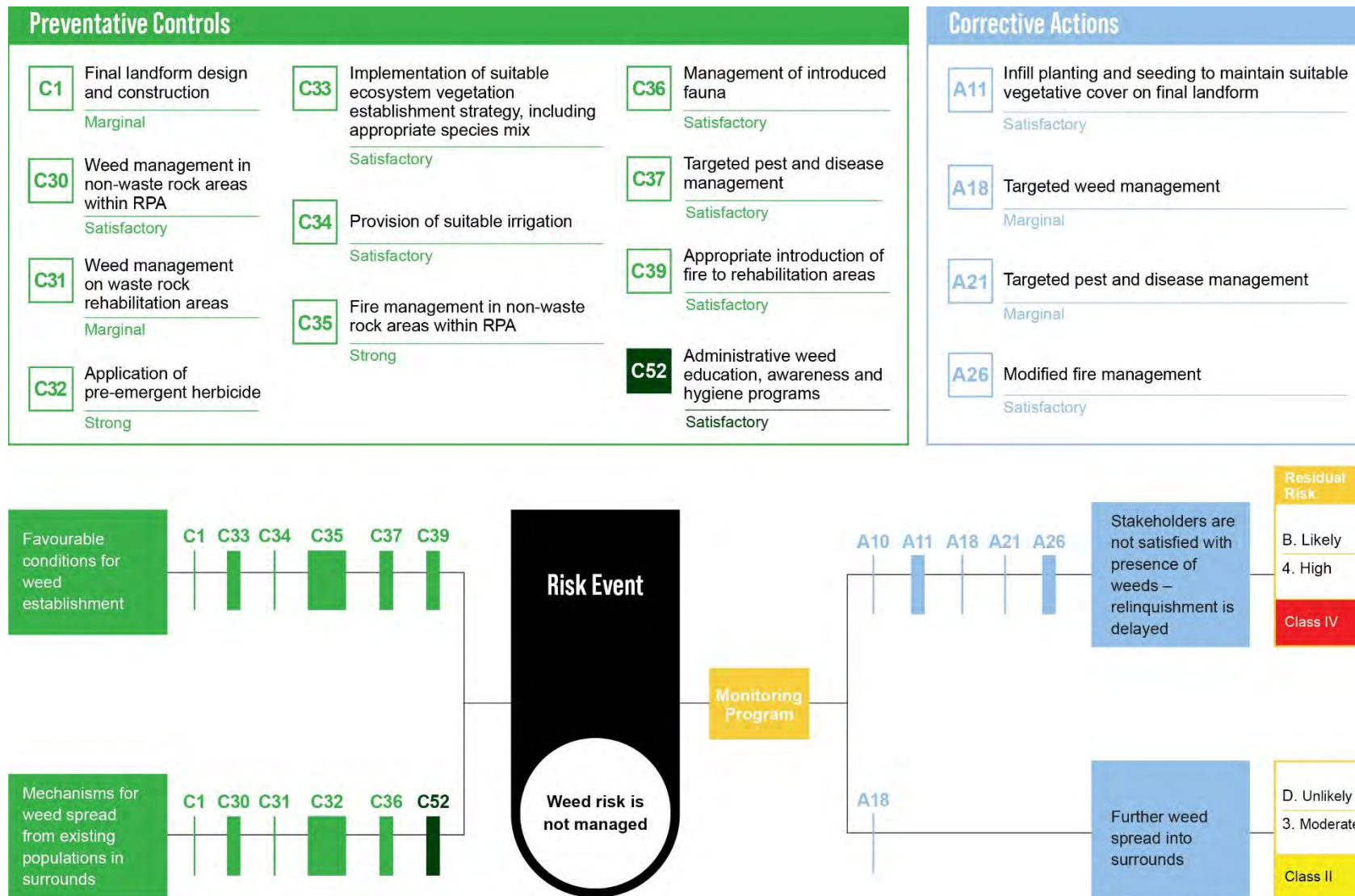
Figure 9-8: Bow-tie diagram for management of weed risk (ES6)
