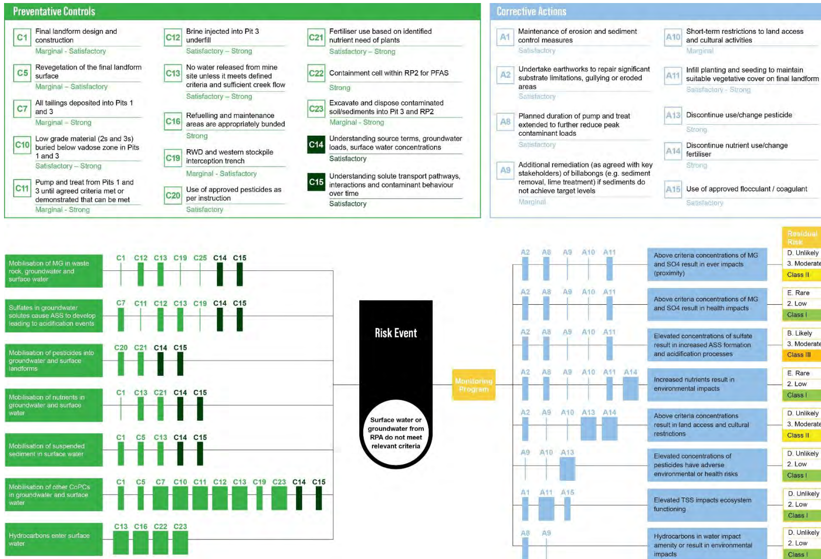
Figure 7-17: Bow-tie diagram for Final Landform and Land Application Areas (WS3)
