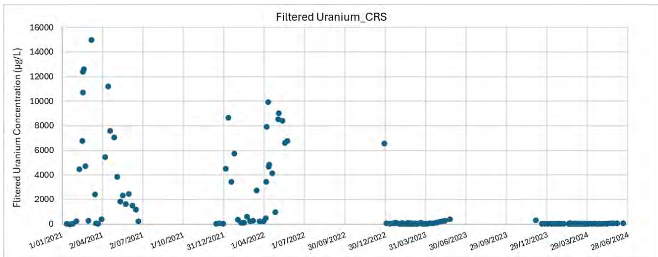
Figure 7-7: Pit 1 - CRS water quality data – Filtered uranium
