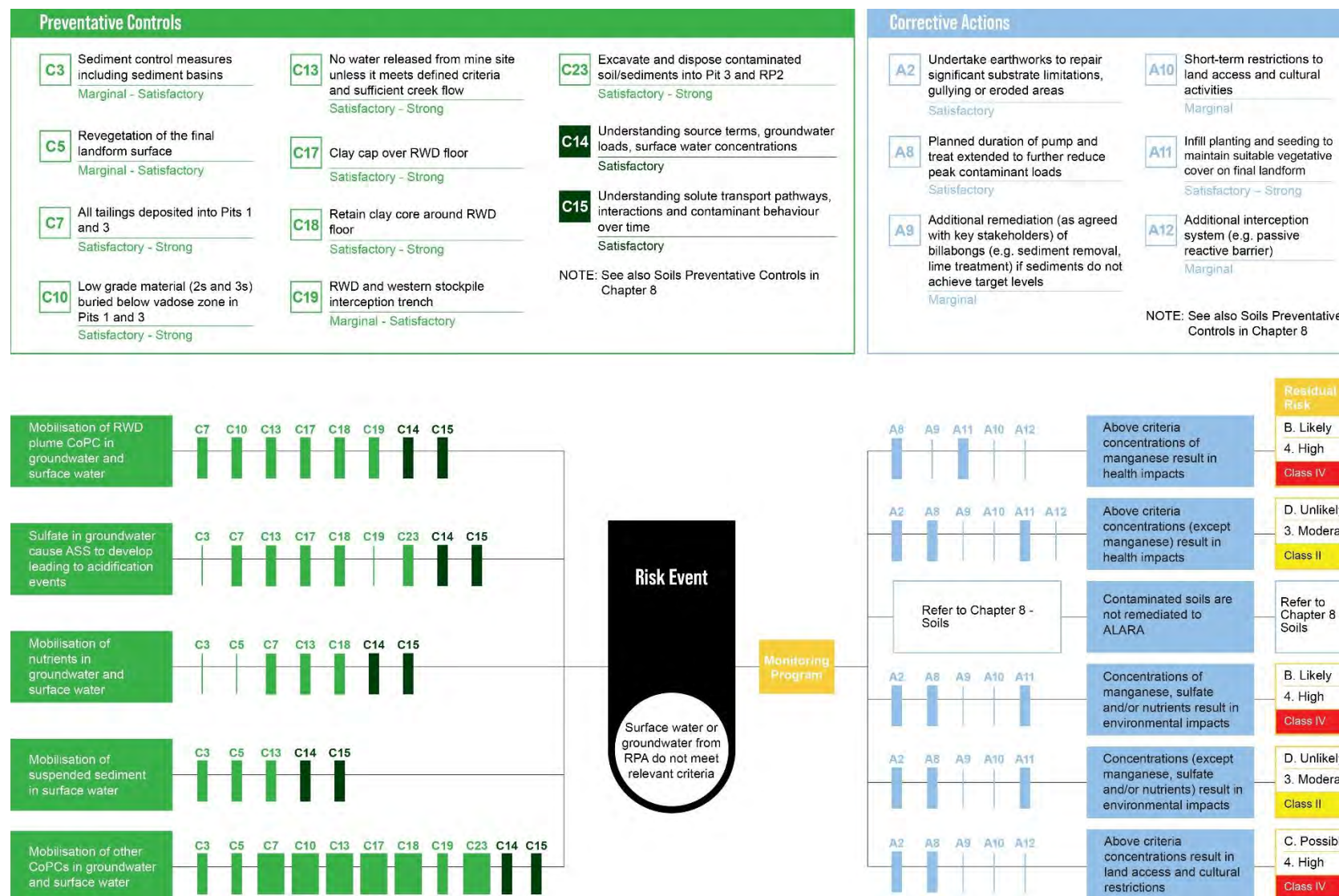
Figure 7-16: Bow-tie diagram for Coonjimba and Gulungul catchments (WS2)
