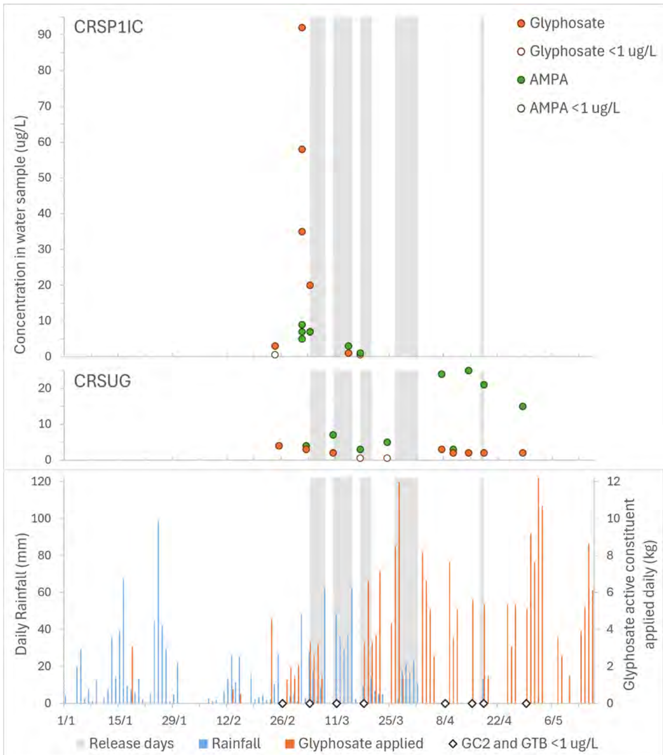
Figure 7-9: Daily rainfall (Jabiru airport) and estimated glyphosate applied daily in the Pit 1/CRS catchment from 1 Jan to 16 May 2024 (bottom). Glyphosate and AMPA concentrations at CRSP1IC and CRSUG (top).
