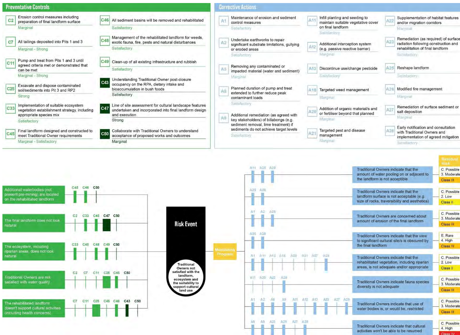
Figure 11-1: Bow-tie diagram for closure criteria – creating a landform that meets Traditional Owner requirements (CL1)
