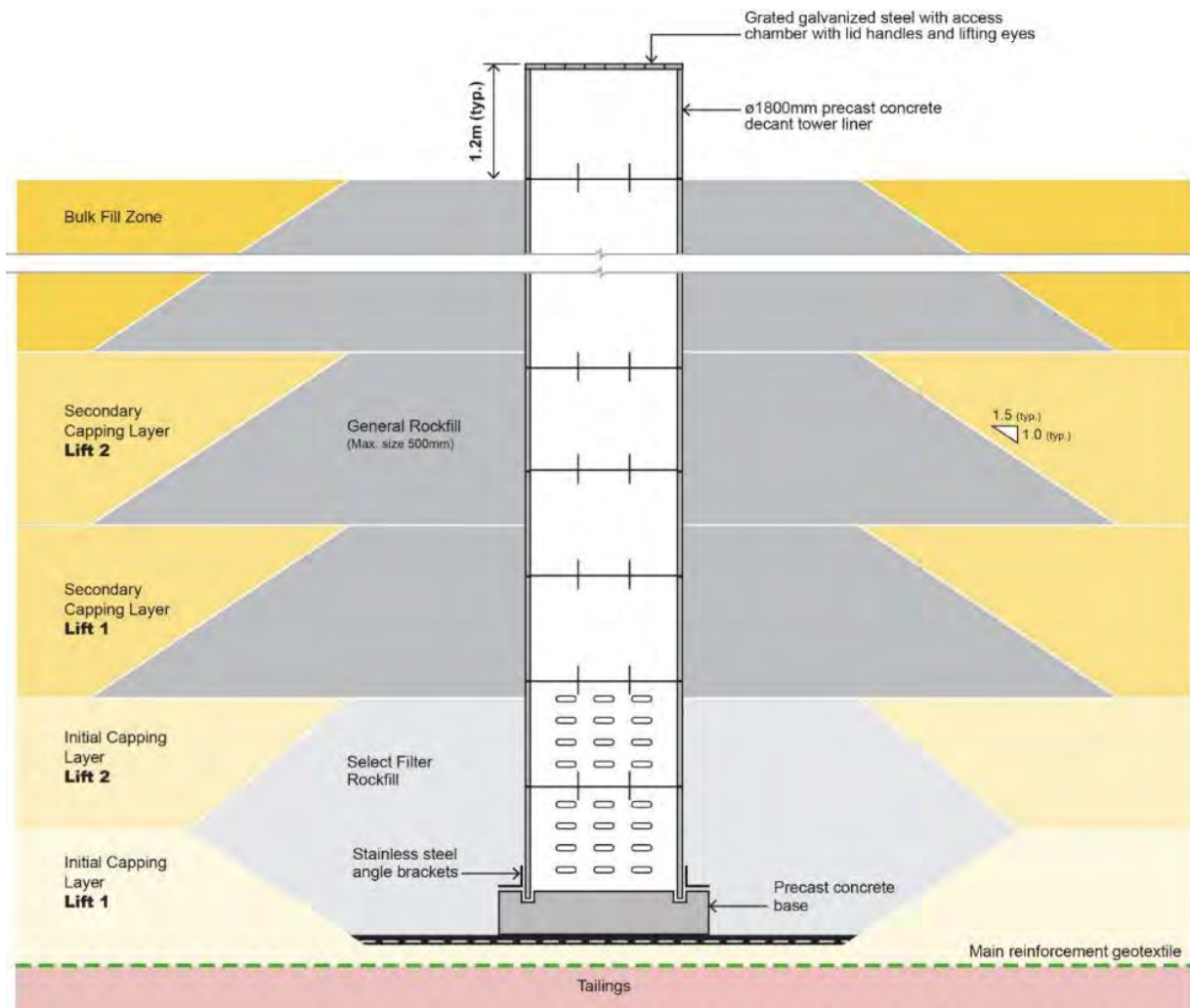
Figure 4-12: Decant well typical section (indicative only – subject to change)
