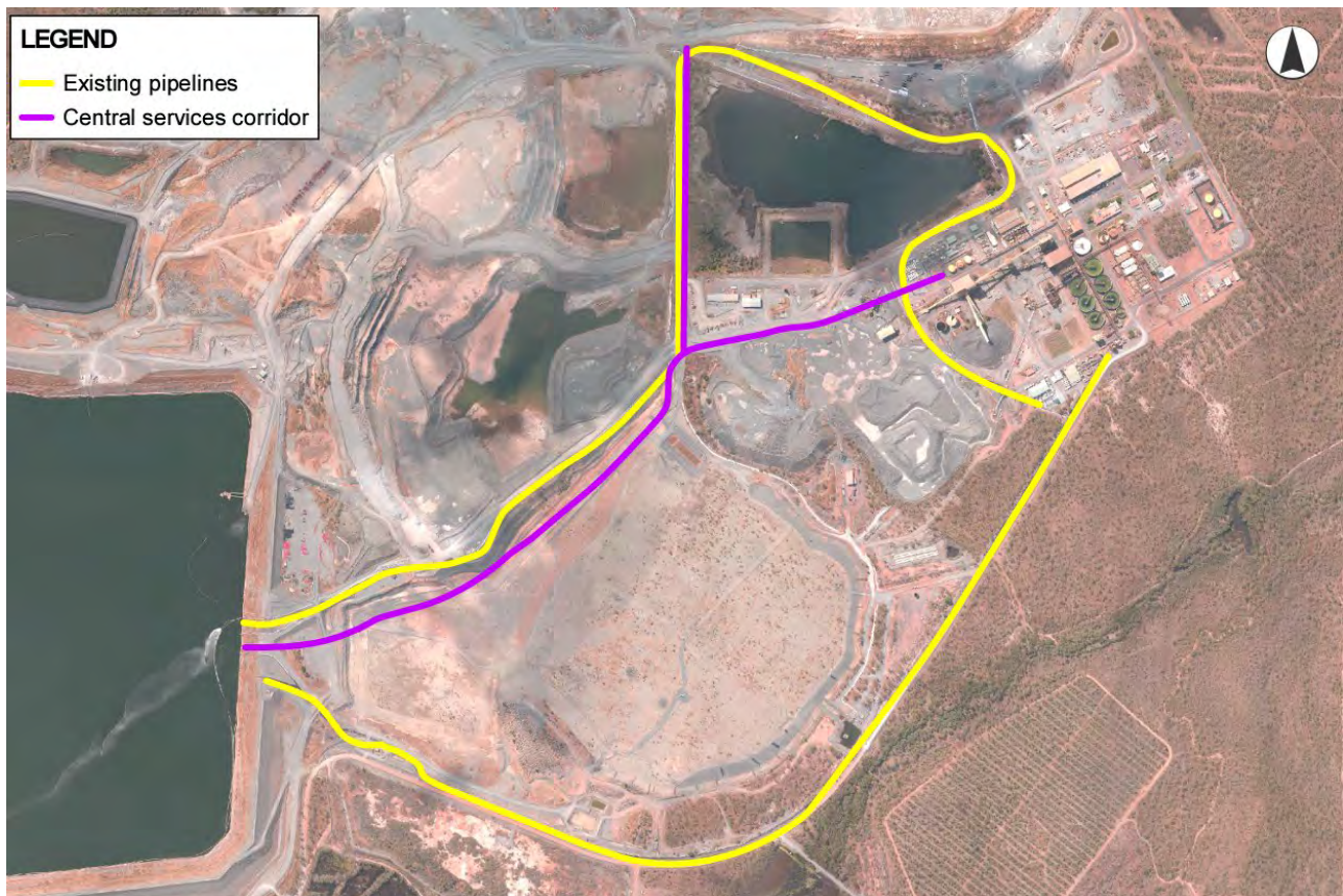
Figure 4-23: Existing pipeline corridors (yellow lines) and proposed central services corridor (purple lines)
