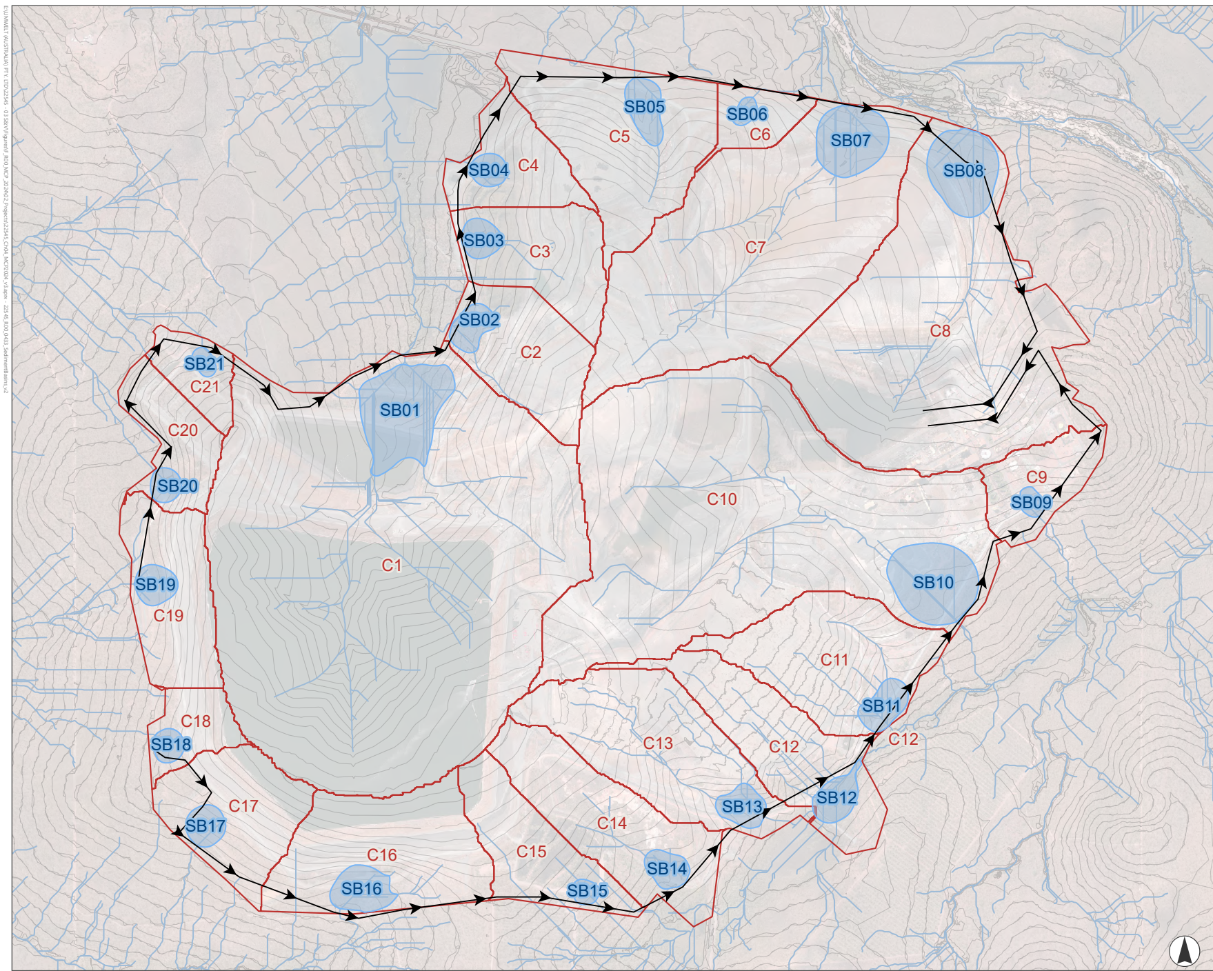
FIGURE 4-32 Sediment Basin and Catchment Arrangement
