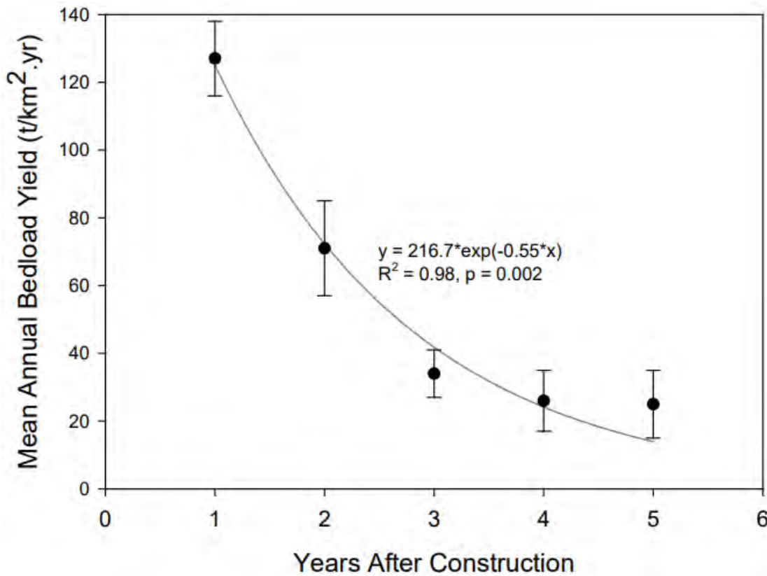
Figure 6-3: Decrease in mean annual bedload yield with time since construction on the TLF (Lowry and Saynor, 2015)
