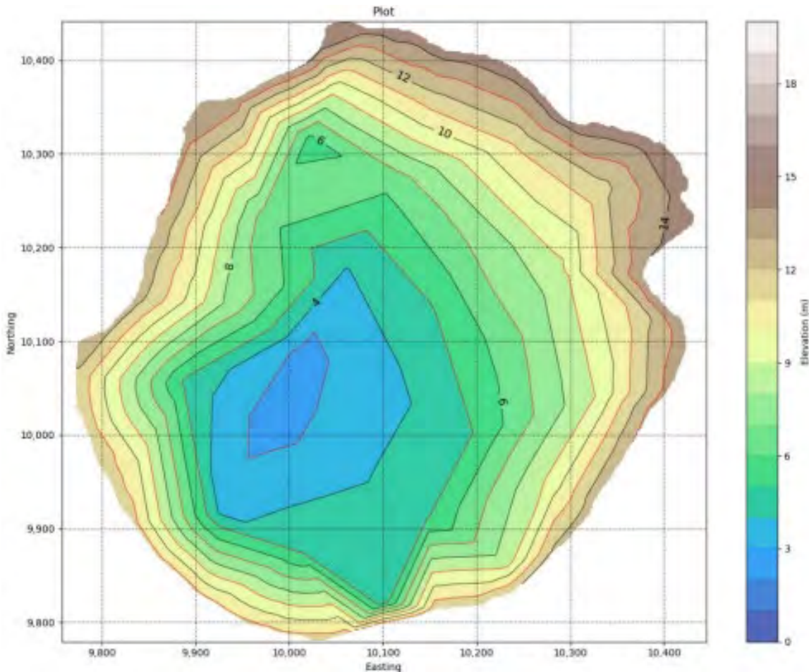
Figure 6-5: Calculated Pit 1 tailings surface as of May 2021 (S. Murphy, per. comms.1 June 2021)
