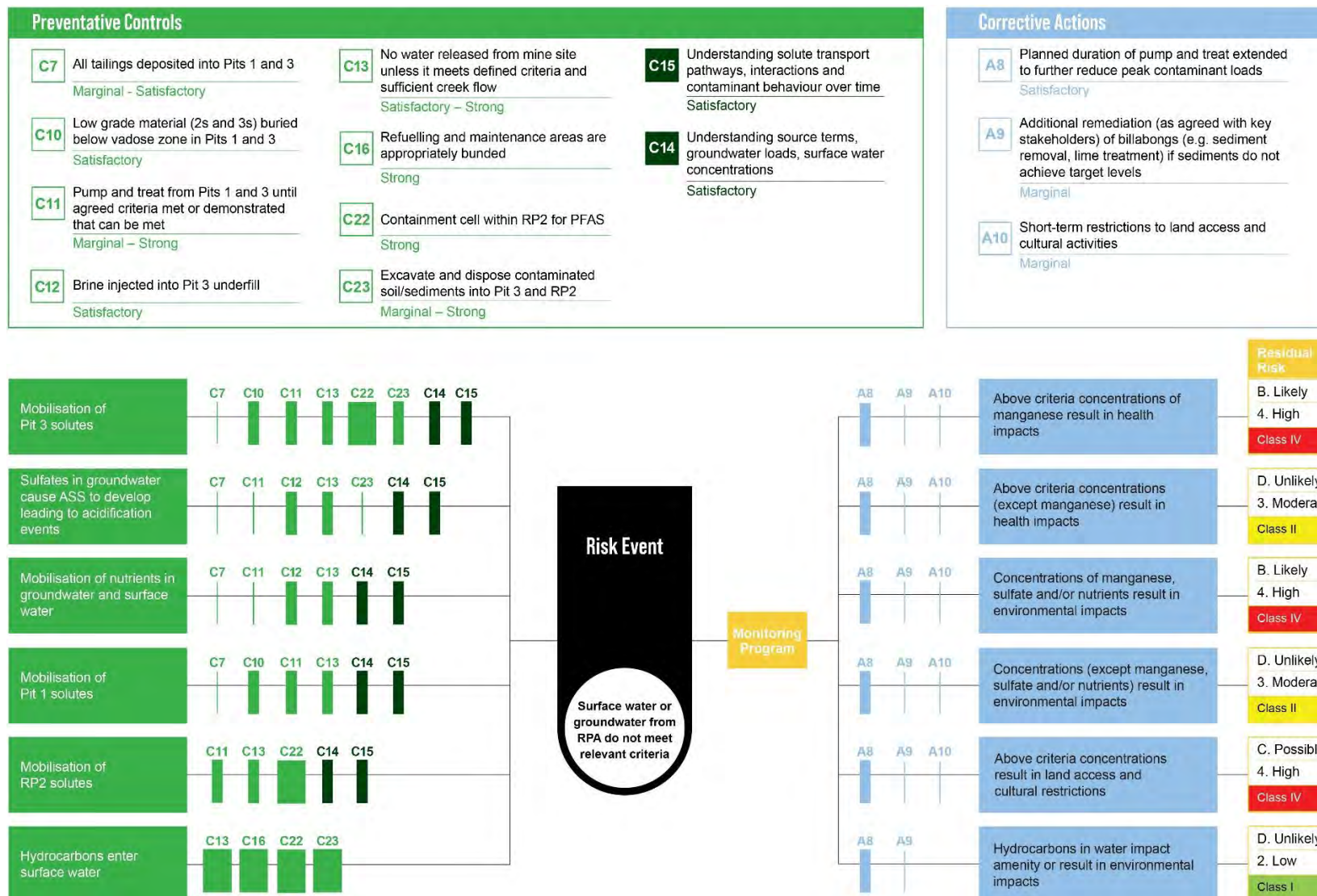
Figure 7-15: Bow-tie diagram for Djalkmarra and Corridor Creek catchments (Pit 1, Pit 3 and RP2) (WS1)
