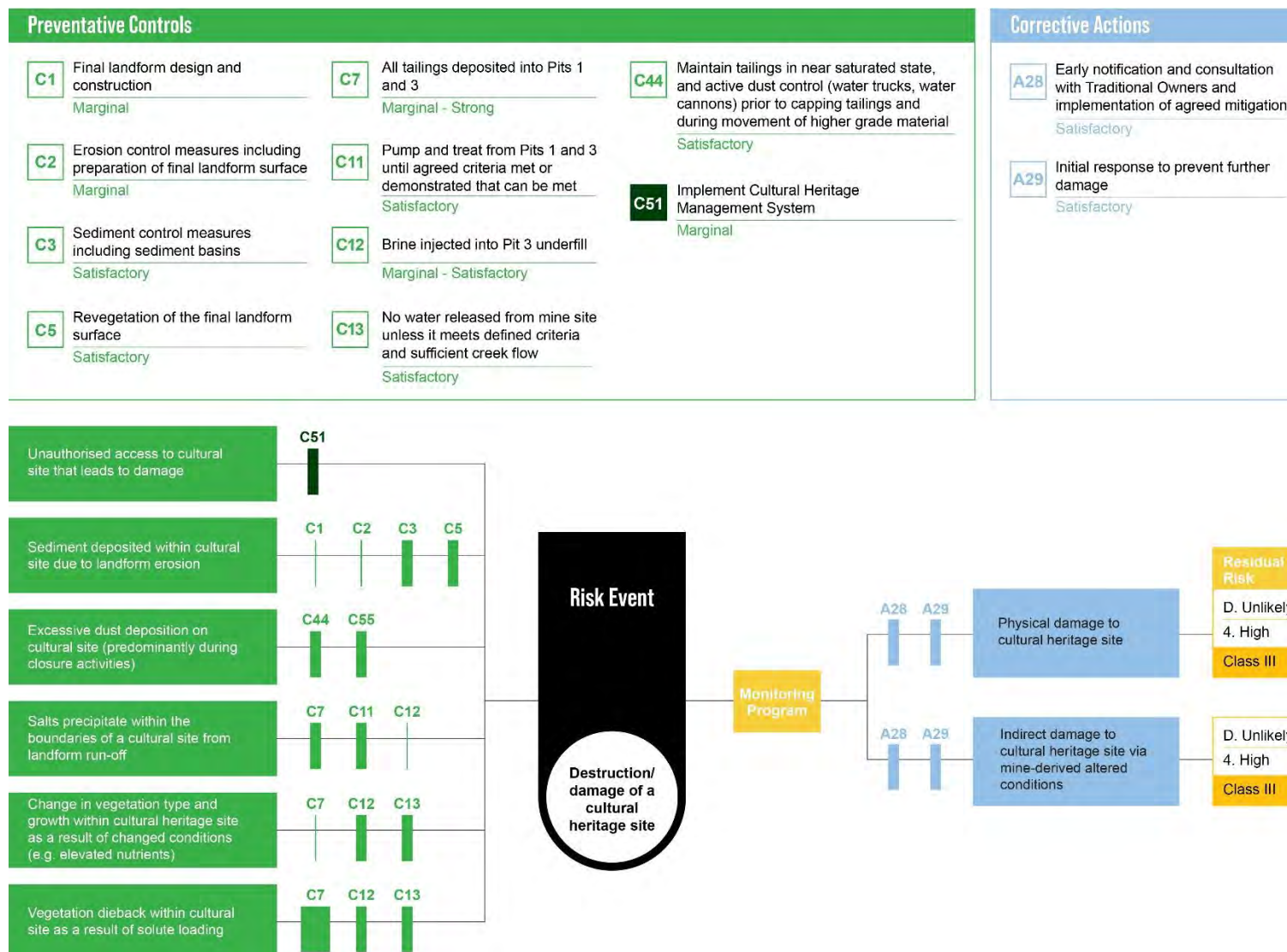
Figure 11-2: Bow-tie diagram for cultural management – to avoid destruction or damage to a cultural site (CL2)
