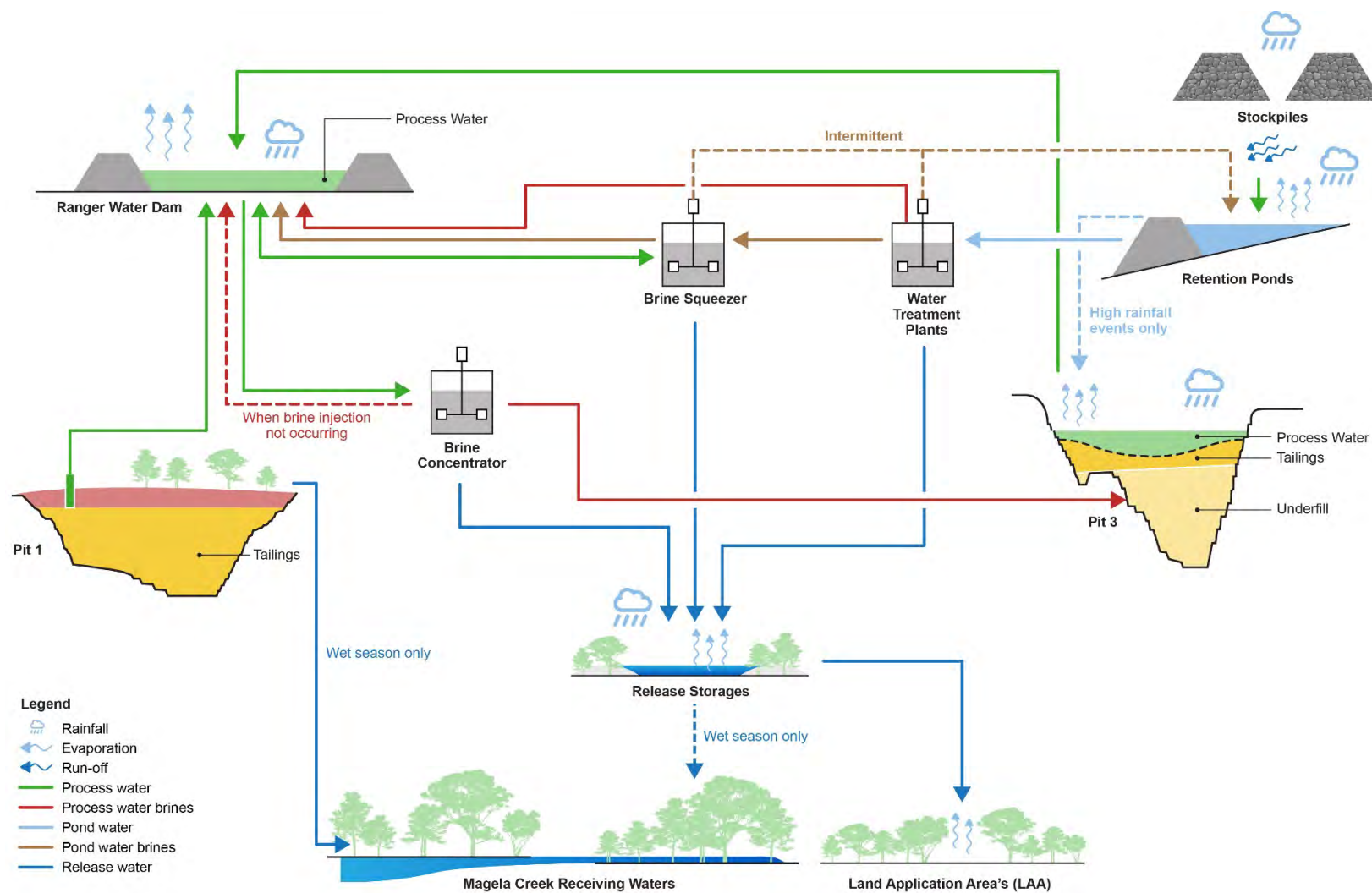
Figure 4-14: Ranger water circuit
