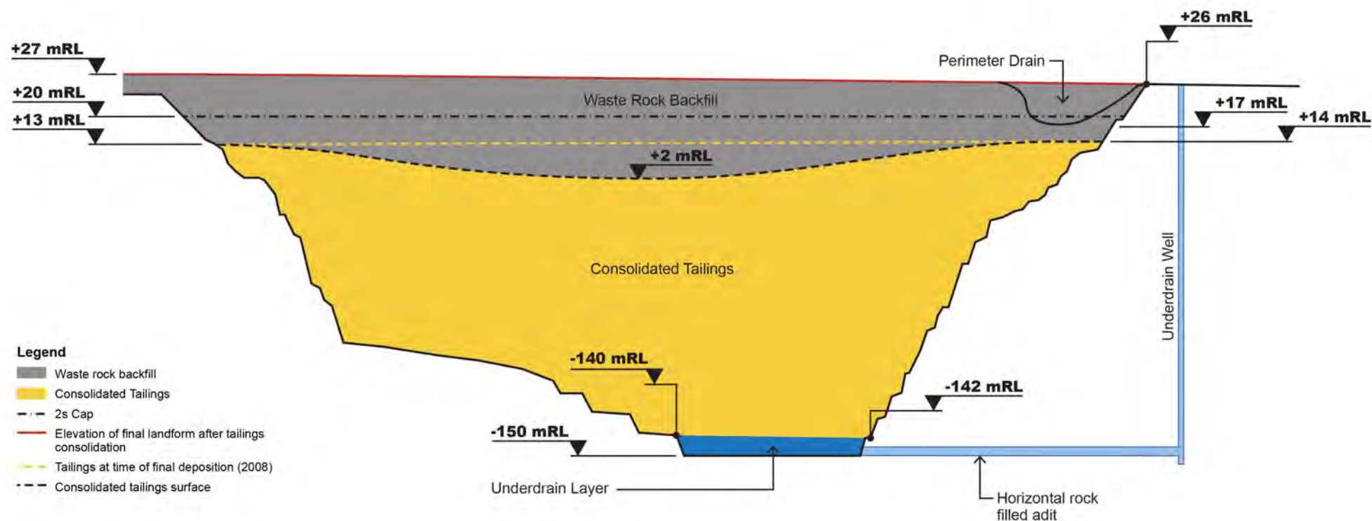
Figure 4-3: Schematic of Pit 1 with key elevations (not to scale)
