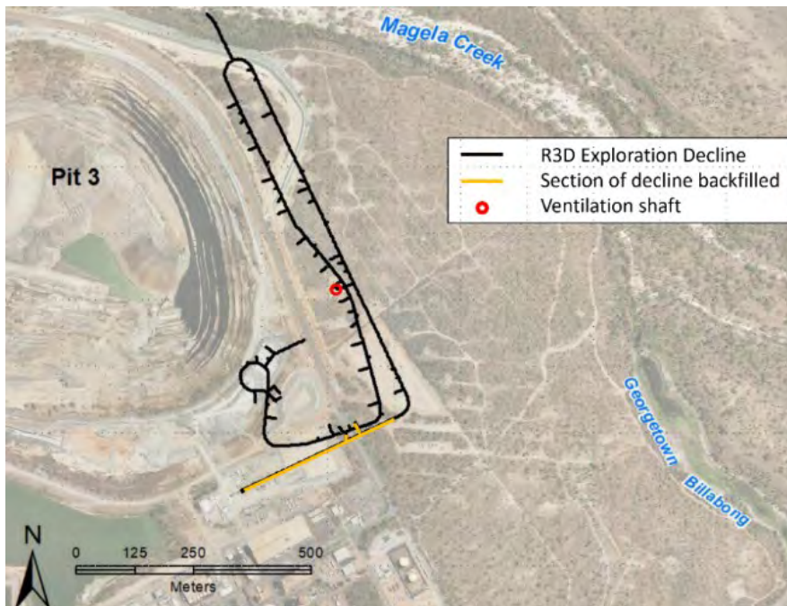
Figure 4-26: Plan view of the R3 Deeps decline
