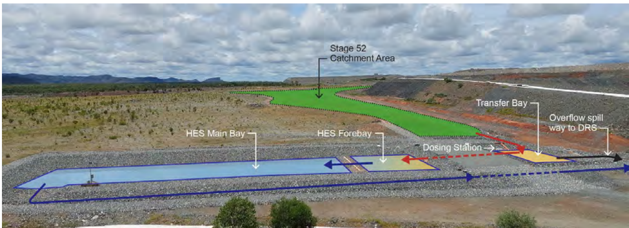
Photo 6-3: Stage 52 HES Basin (31 January 2023)
