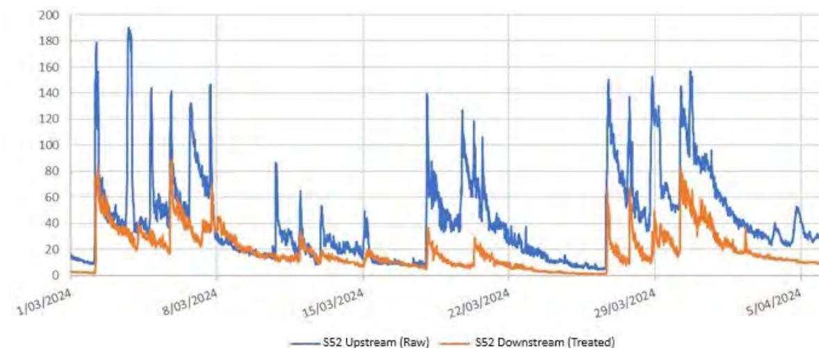
Figure 6-4: Stage 52 Inflow vs Outflow Turbidity (March 2024)
