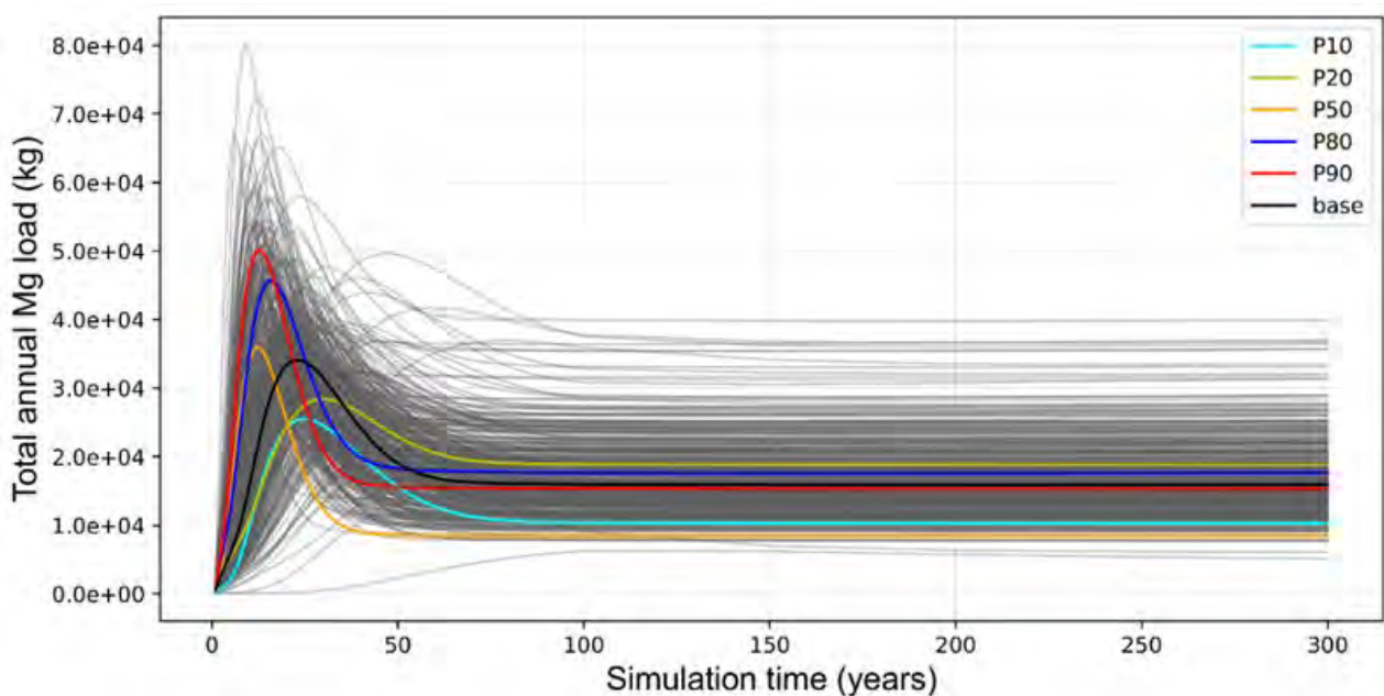
Figure 7-4: Horsetail plot of Pit 3 uncertainty analysis modelled magnesium loads from Pit 3 sources
