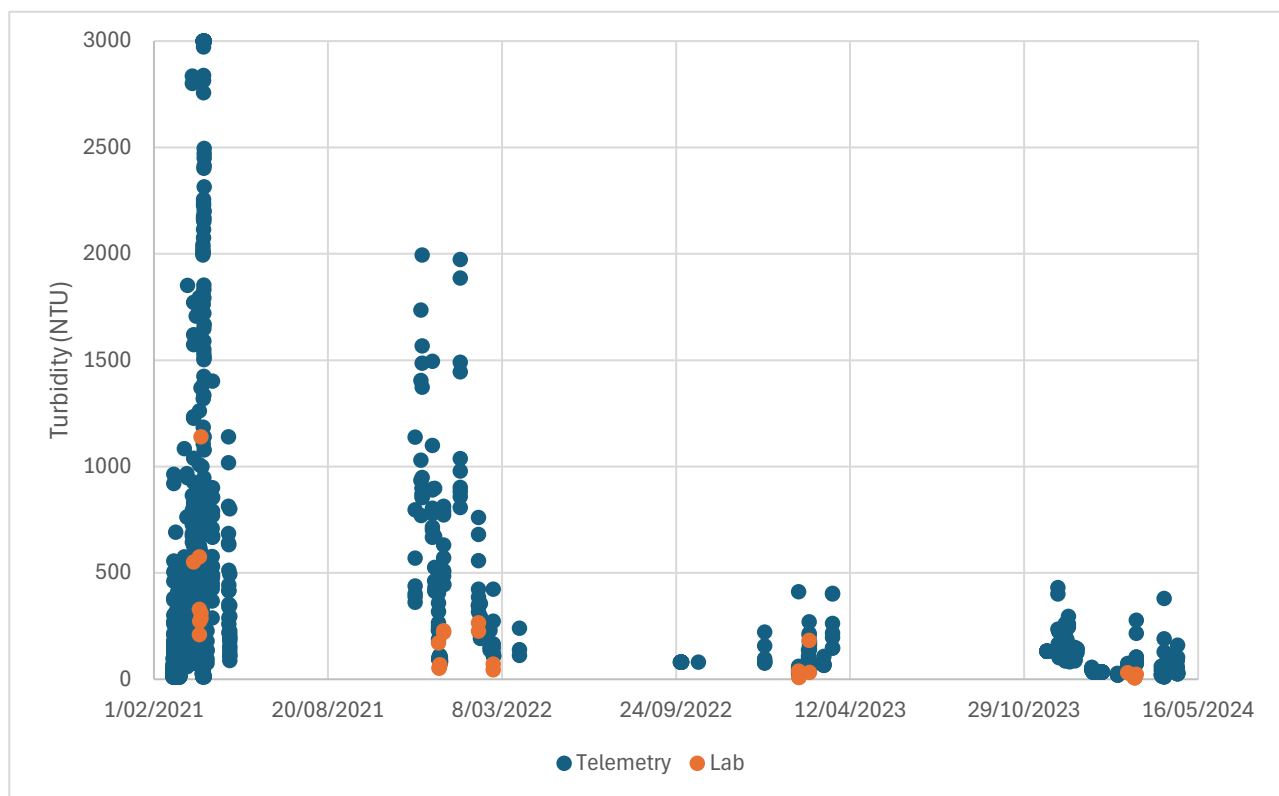
Figure 6-2: Pit 1 inlet channel telemetry and lab turbidity
