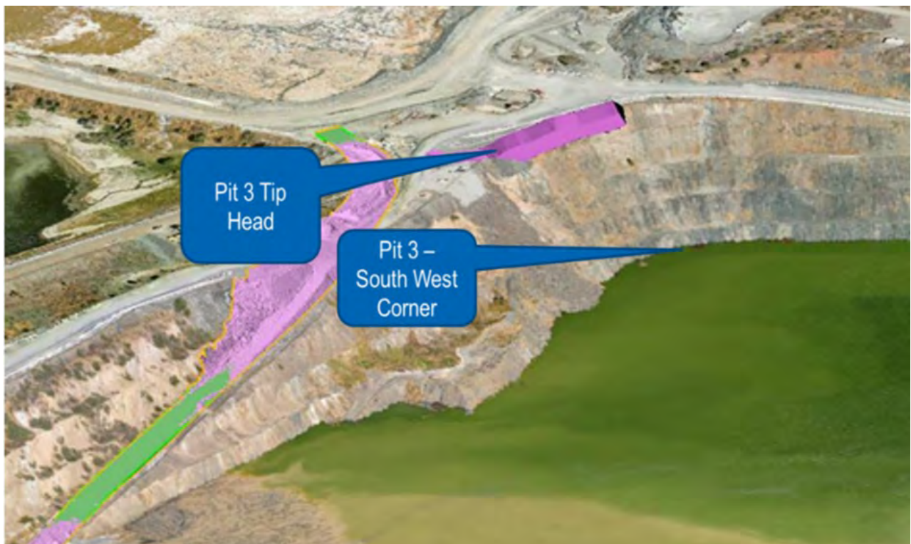
Figure 4-10: View of the Pit 3 wall for proposed tip head (south-west view)
