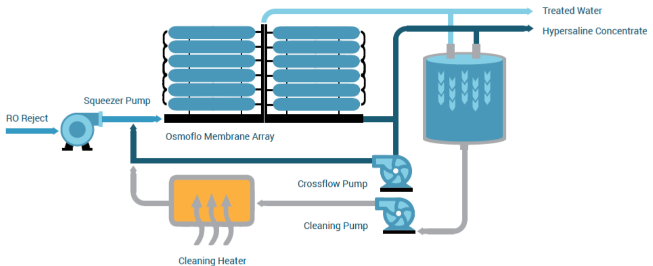
Figure 2-1: Brine Squeezer process flow diagram (source: http://www.osmoflo.com/ )
