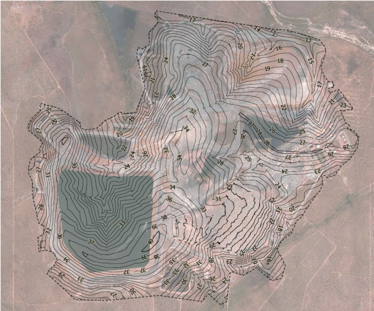
Figure 4: Final landform boundary and contours (metres reference level; mRL)
